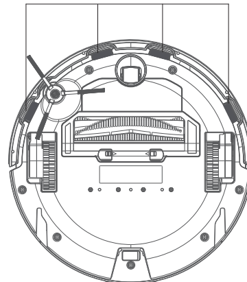
Cliff sensor
